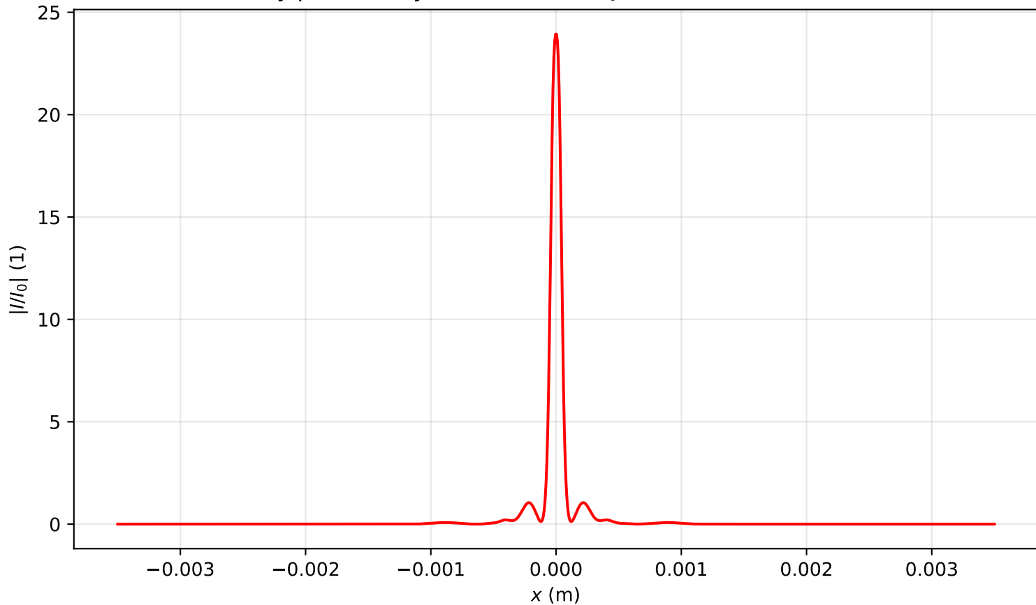
Intensity profile I(x, y = 0, z = 1.194)/I_0 , P_{in}=4.5P_{cr} , artificial time
